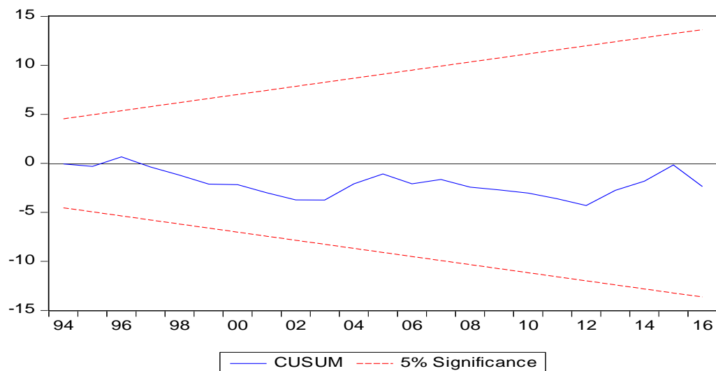
Fig. 1: CUSUM Stability Test
